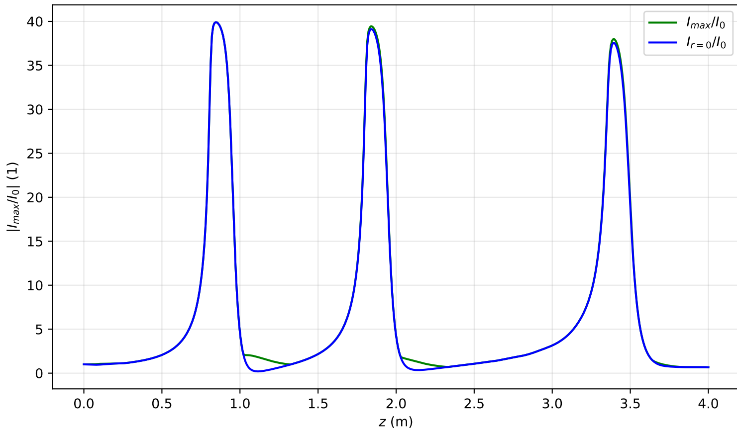
I_{max}(x = 0, y = 0, z)/I_0 , P_{in}=2.7P_{cr} , noisy input, artificial time
